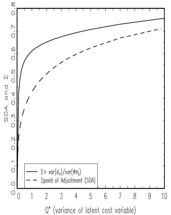
D) SOA and \Sigma as a function of Q^*
