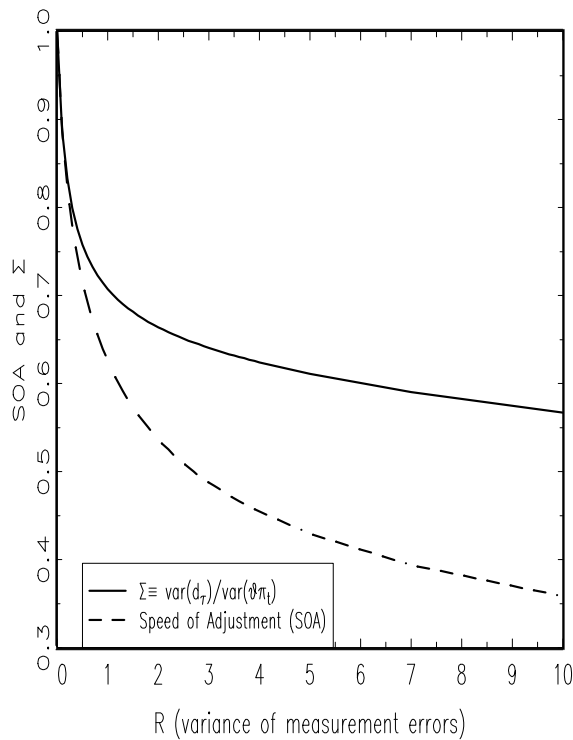
C) SOA and \Sigma as a function of R
