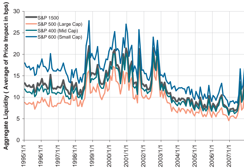
Figure 6: Monthly cross-sectional averages of price impact coefficients \hat{\lambda}_i of stocks in the S&P 1500 and sub-components between January 1995 and December 2007, based on daily time-series regressions for each stock i within each month: R_{i,t} = \hat{c}_i + \hat{\lambda}_i \cdot \text{Sgn}(t) \log(v_{i,t} p_{i,t}) + \epsilon_{i,t} where \text{Sgn}(t) \log(v_{i,t} p_{i,t}) is the signed volume of security i on date t and the sign is determined by “tick test” applied to daily returns. Components of these indexes are based on the memberships on the last day of the previous month.
