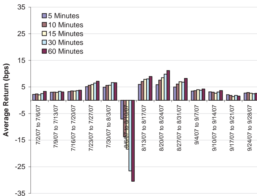
Figure 7: The average return for the contrarian strategy applied to 5-minute returns from July 2, 2007 to September 28, 2007. Each day is divided into non-overlapping 5-minute intervals, and positions are established based on lagged 5-minute returns and then held for 5, 10, 15, 30, or 60 minutes. The average return for each holding period is calculated for each week during this sample. No overnight positions are allowed, initial positions are established at 9:40am each day and all positions are closed at 4:00pm. Components of the S&P 1500 are based on memberships as of the last day of the previous month.
