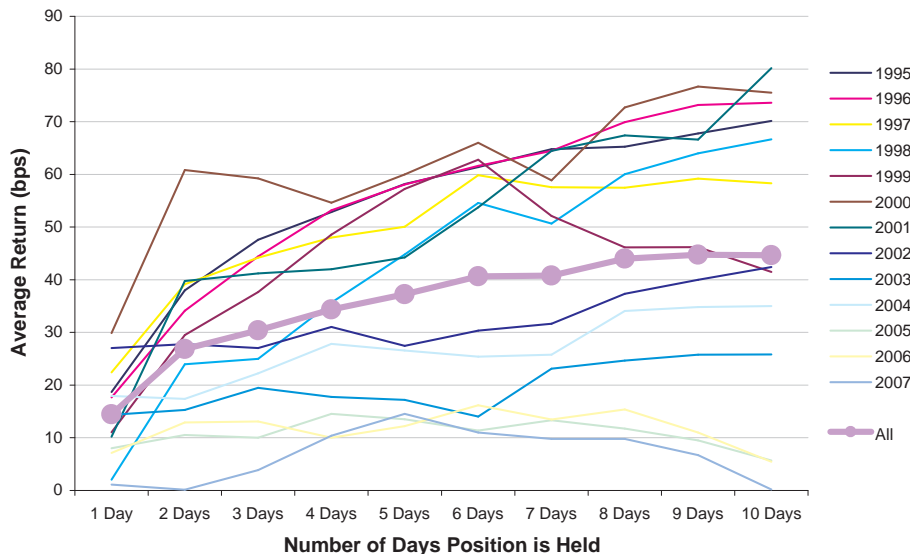
Figure 5: Average return of the contrarian strategy when portfolios are constructed based on 1-day lagged returns and positions are held for 1 to 10 days for January 3, 1995 to December 31, 2007. A return is assigned to the year in which the position was established and averages are then calculated for different holding periods. Components of the S&P 1500 are based on memberships as of the last day of the previous month.
